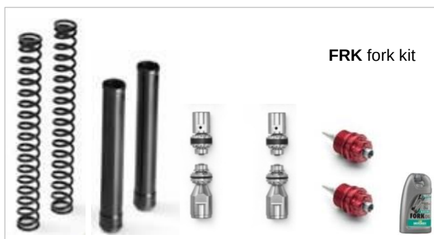
fork 46 without OEM bottom compression valve
